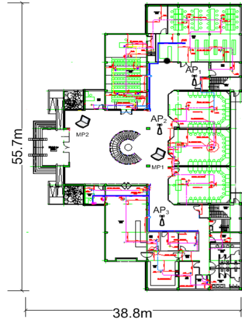
Fig. 8. Floor plan of the area where the DiP experiment was performed.
