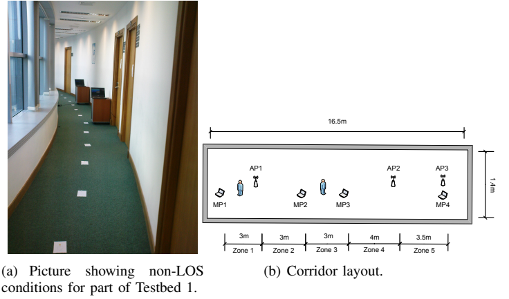
Fig. 17. Testbed 1: The corridor is separated by laptops and APs into five zones.
