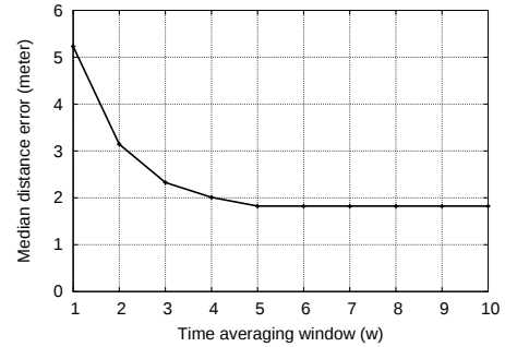
Fig. 14. Median distance error of the continuous space estimates versus the time averaging window size ( w ).
