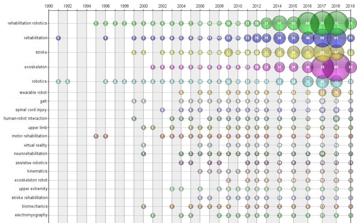
Fig. 2. Bubble chart of top 20 author keywords by year. The size of the bubble represents the number of publications employing that keyword.
