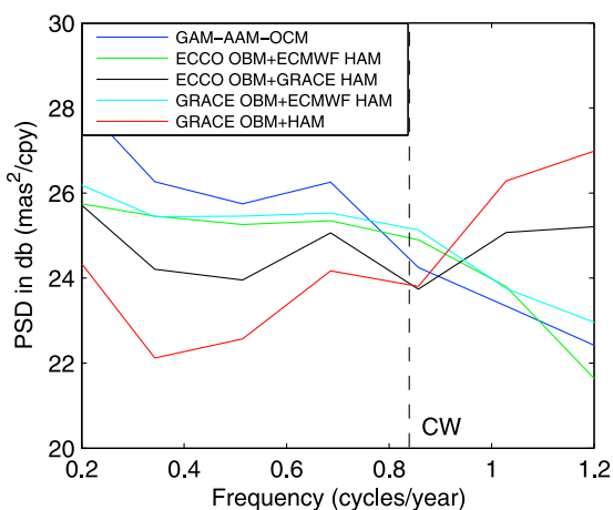
Figure 6. Power spectral density ( \text{mas}^2/\text{cpy} ) for polar motion P_x + i P_y of the geodetic observation residuals of GAM-AAM-OCM (blue line) with GRACE and models' estimates. A mean, trend, and seasonal signals at the annual and semiannual frequencies have been removed from all time series prior to the fast Fourier transform analysis. The vertical dashed line is at the Chandler wobble period.
