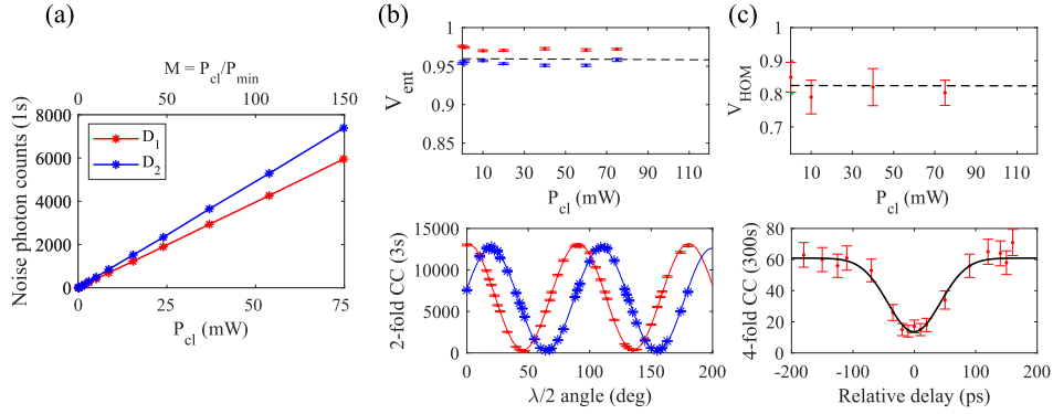
Fig. 2. (a) SpRS noise photon count rate in the Bell state measurement (BSM) detectors D_1 and D_2 as a function of the classical launch power P_{cl} and the ratio M to the minimum power P_{min} needed to operate a single 400-Gbps channel. (b) Bob's entanglement distribution visibility V_{ent} over 15.0 km to the BSM node versus P_{cl} (top) and the corresponding two-fold coincidence count (CC) non-local interference fringe measured in the vertical (red) and anti-diagonal (blue) bases for P_{cl} = 74 mW (bottom). (c) Hong-Ou-Mandel interference visibility V_{HOM} over 30.2 km between heralded photons from Alice and Bob's sources versus P_{cl} (top) and the corresponding four-fold coincidence interference fringe when P_{cl} = 74 mW (bottom). The dashed lines show the predictions of our theoretical model [48] (see supp. materials).
