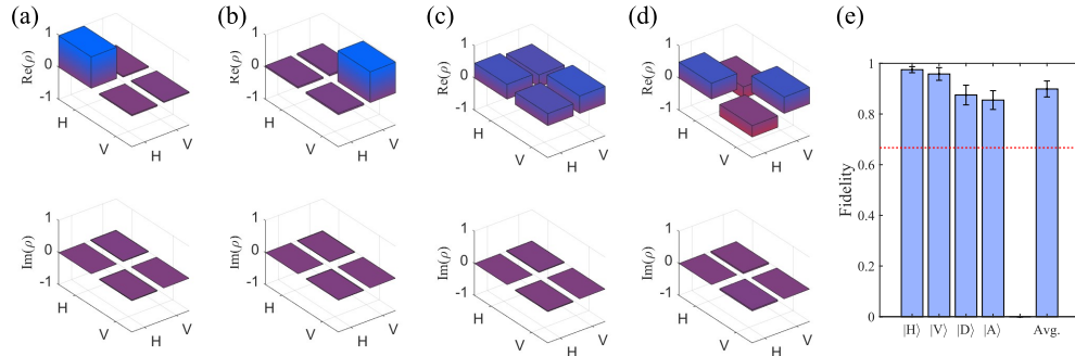
Fig. 4. Real and imaginary components of the density matrices obtained by single-qubit quantum state tomography on Bob's target photon, conditioned on a successful BSM, whilst the launch power of the 400-Gbps C-band signal into the 30.2-km fiber is set to 74 mW. (a-d) show the results for Alice transmitting |\psi\rangle_A = |H\rangle , |V\rangle , |D\rangle , and |A\rangle , respectively. (e) The fidelity of Bob's density matrix to Alice's ideally prepared qubit and the calculated average fidelity. The dotted line shows the F = 2/3 limit for the highest fidelity achievable using only classical physics-based methods [52].
