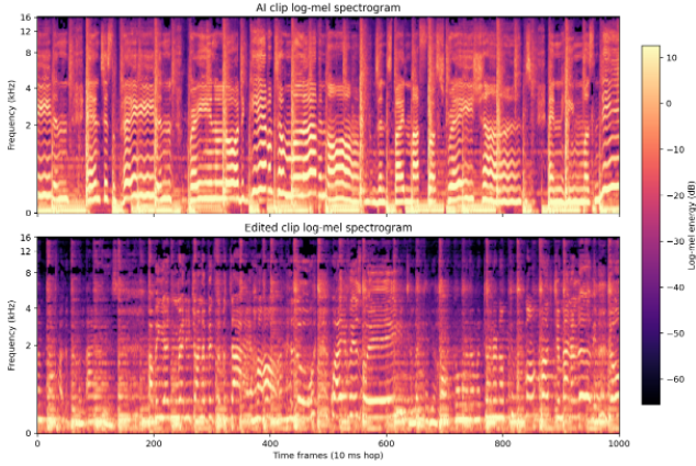
Figure 1: Log-Mel spectrogram comparison for an AI-generated clip and an edited clip from the same reference song.
