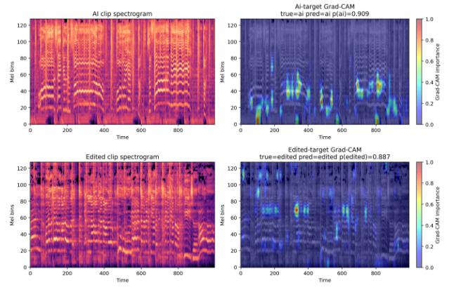
Figure 2: Grad-CAM visualization for the same-song AI/edited pair.
