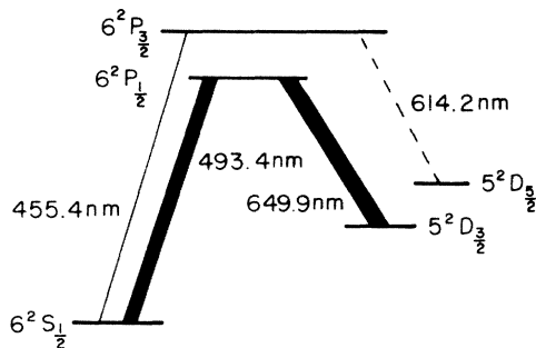
FIG. 1. Level structure of \text{Ba}^+ . The shelf level is the 5^2D_{5/2} state. The laser excitation is shown by the bold lines; the lamp excitation is indicated by the light solid line while the subsequent decay into the shelf level is indicated by the dashed line.
