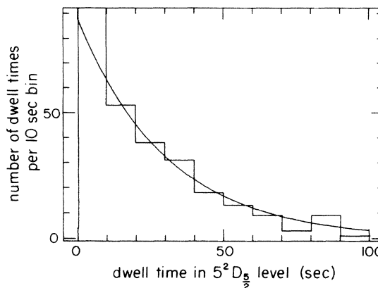
FIG. 3. Histogram of distribution of dwell times in the shelf level for 203 "off" times. A fitted theoretical (exponential) distribution for a metastable lifetime of 30 sec is superposed on the experimental histogram.
